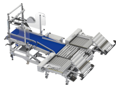
CM Case Management with Case Flap Folder Module
